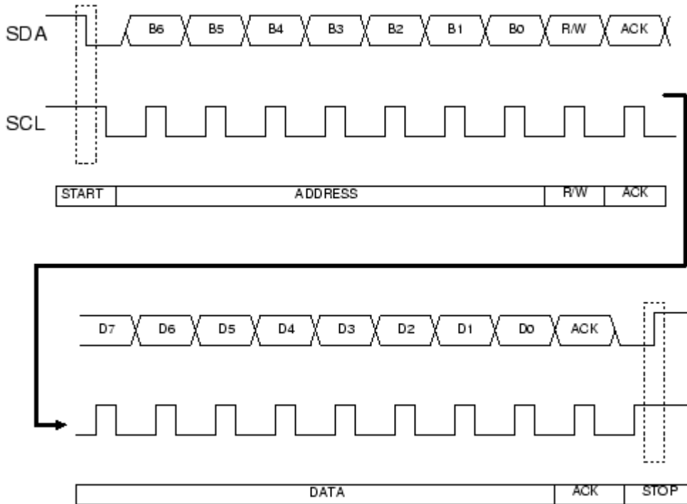
I2C Tutorial : Typical SDA and SCL signals
